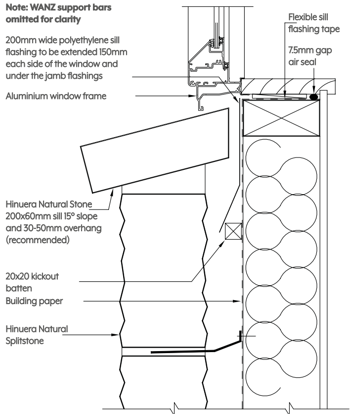
Figure 4: Hinuera Natural Stone Window Sill Detail
