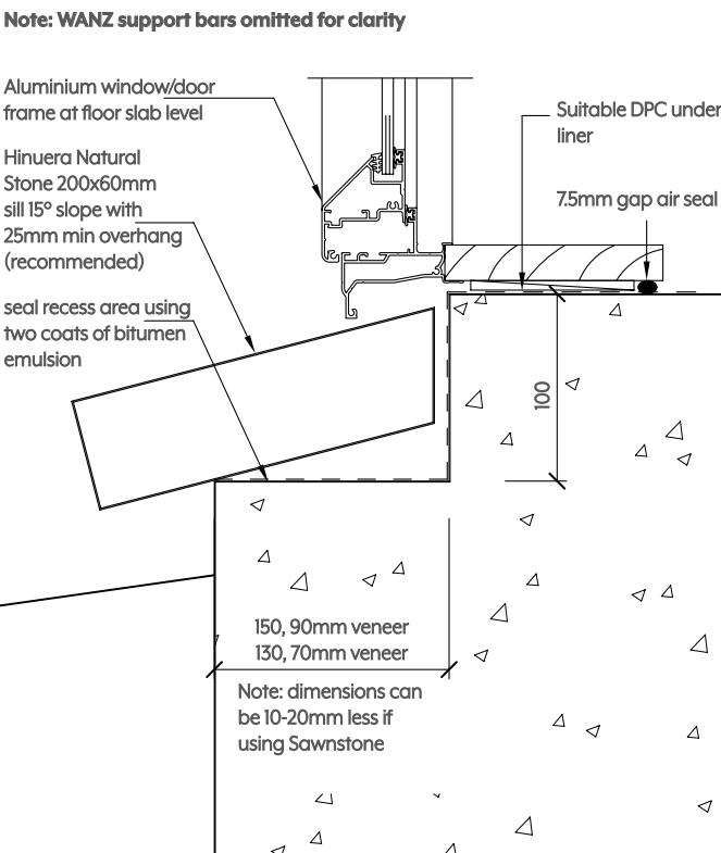
Figure 5: Hinuera Natural Stone Window/Door Sill Detail
