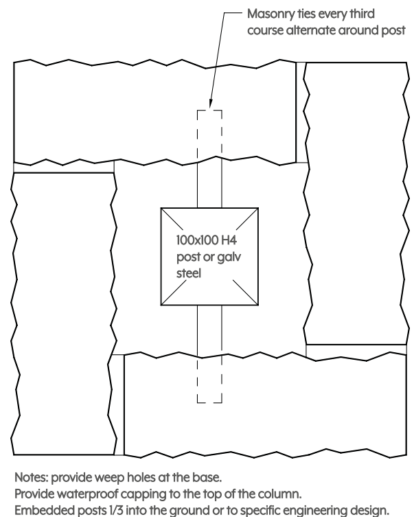
Figure 14: Hinuera Natural Stone Typical Column Detail
